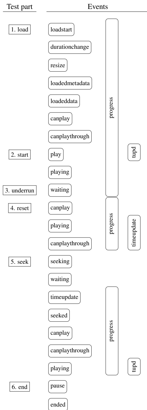
Figure 1: Specification conform event sequence. Fired during loading (1), playing (2), buffer under-run start (3) and end (4), seeking (5), and video end (6). Horizontally shown events are fired once in the given order, vertical entries represent events fired repeatedly.
